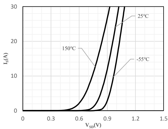
Fig 6 Body-Diode Characteristics
